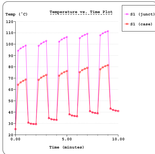
Figure 5: Temperature vs. time graph
