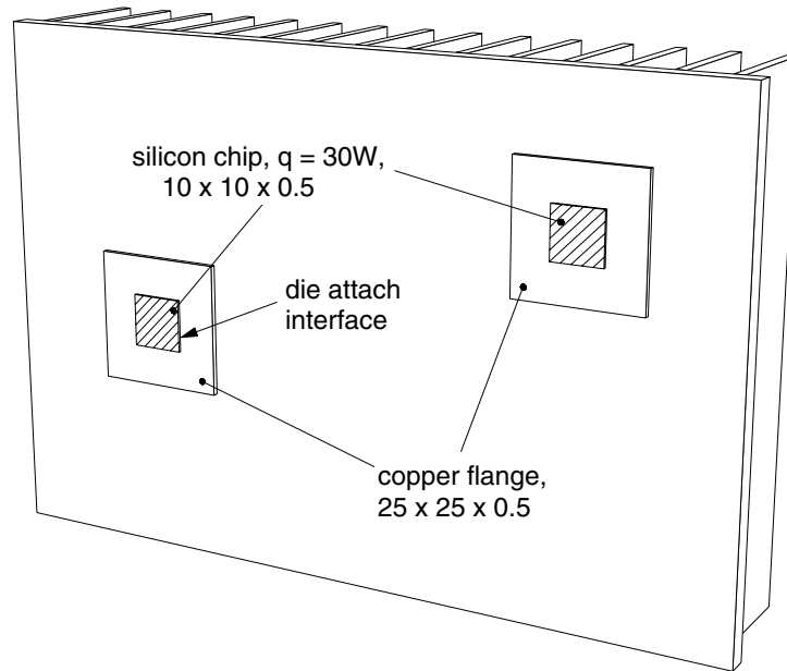
Figure 8: Heat sink with two chip stackups
