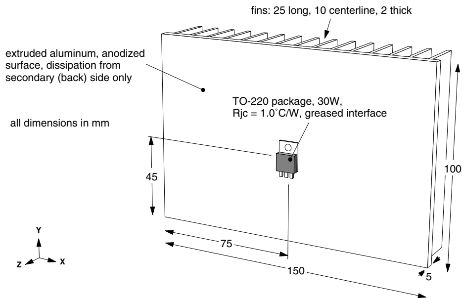
Figure 1: Basic heat sink model
