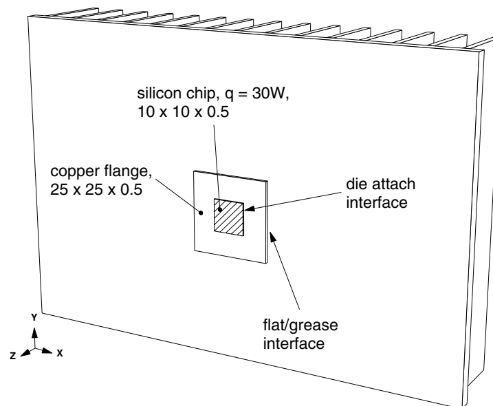
Figure 6: Chip stackup on heat sink
