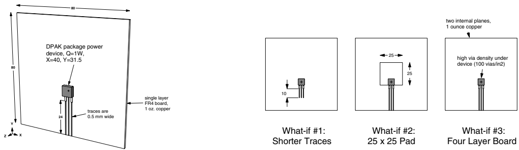
Simple DPAK device model
