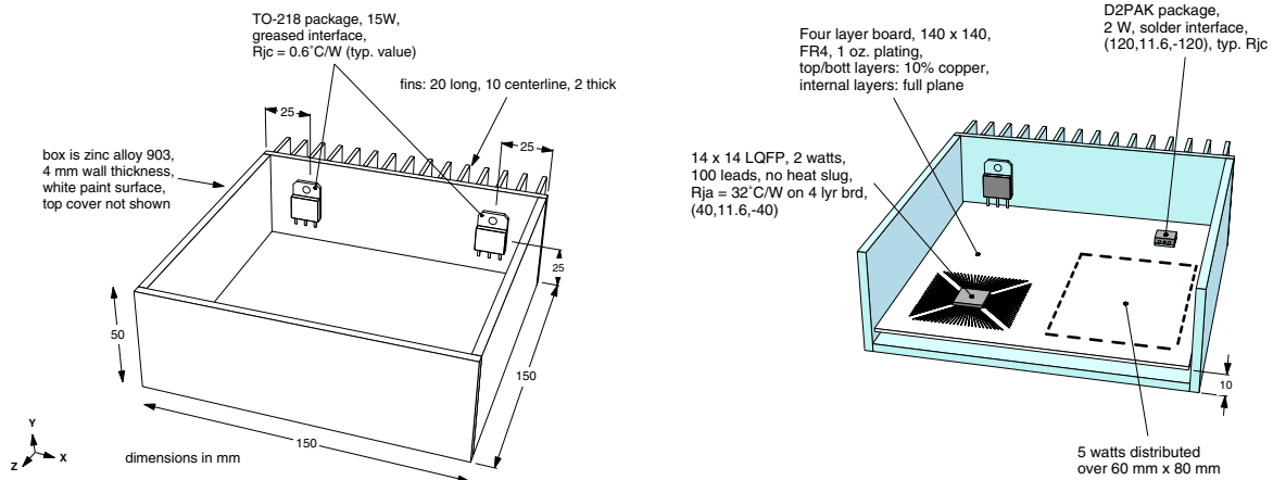
Basic finned box
