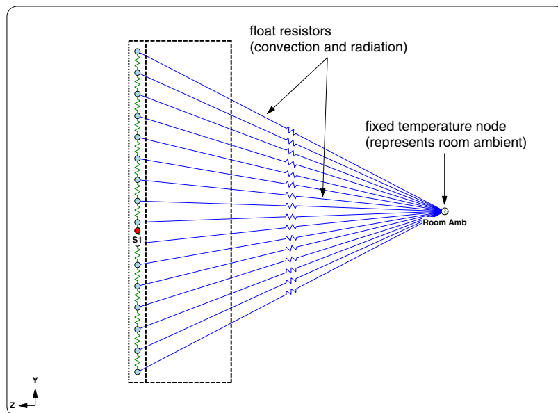
Figure 3: Fixed node and float resistors
