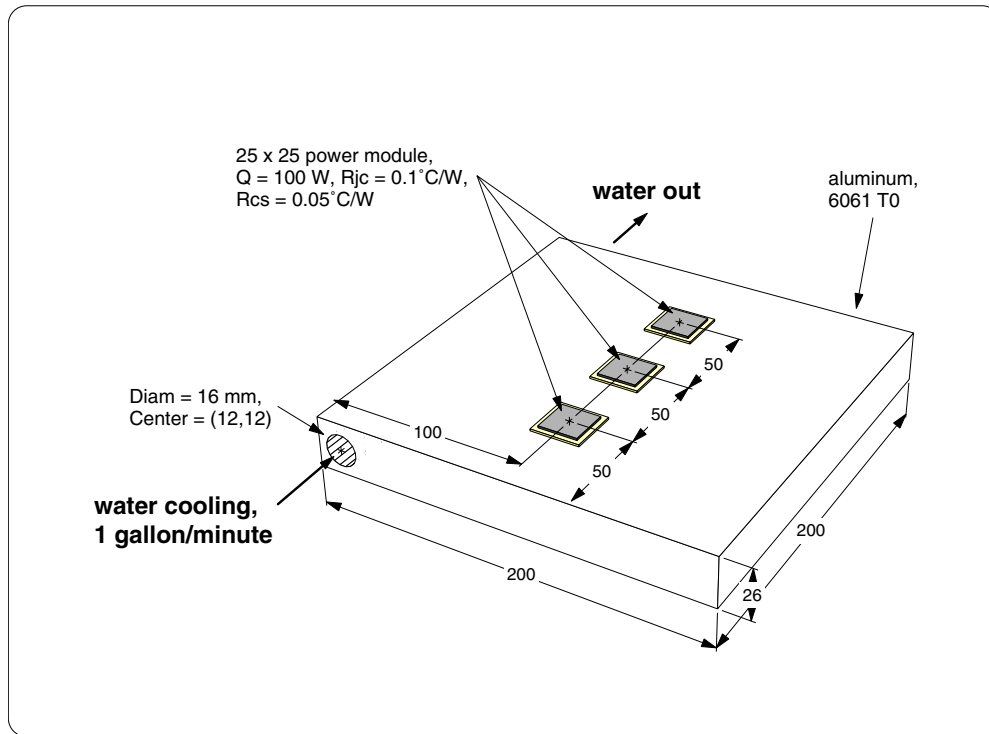
Figure 8: Cold plate model, part 1
