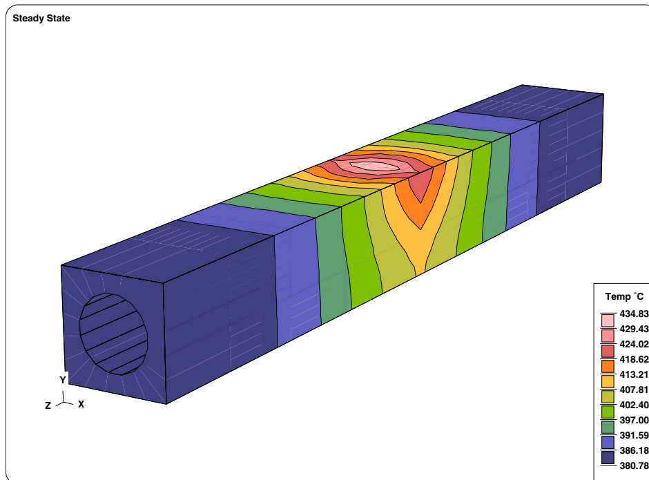
Figure 6: Temperature contours
