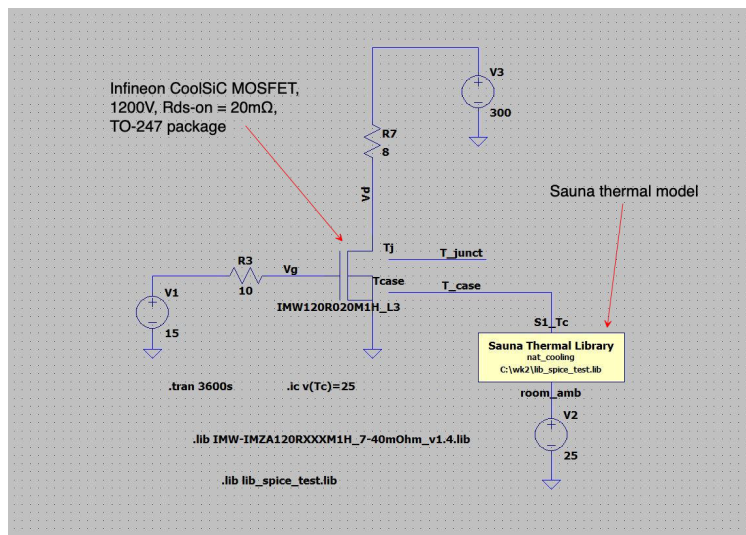
Co-simulation with Infineon CoolSiC MOSFET
