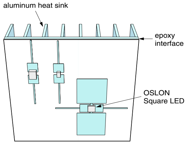
Multilayer board with high power LED, heat sink
